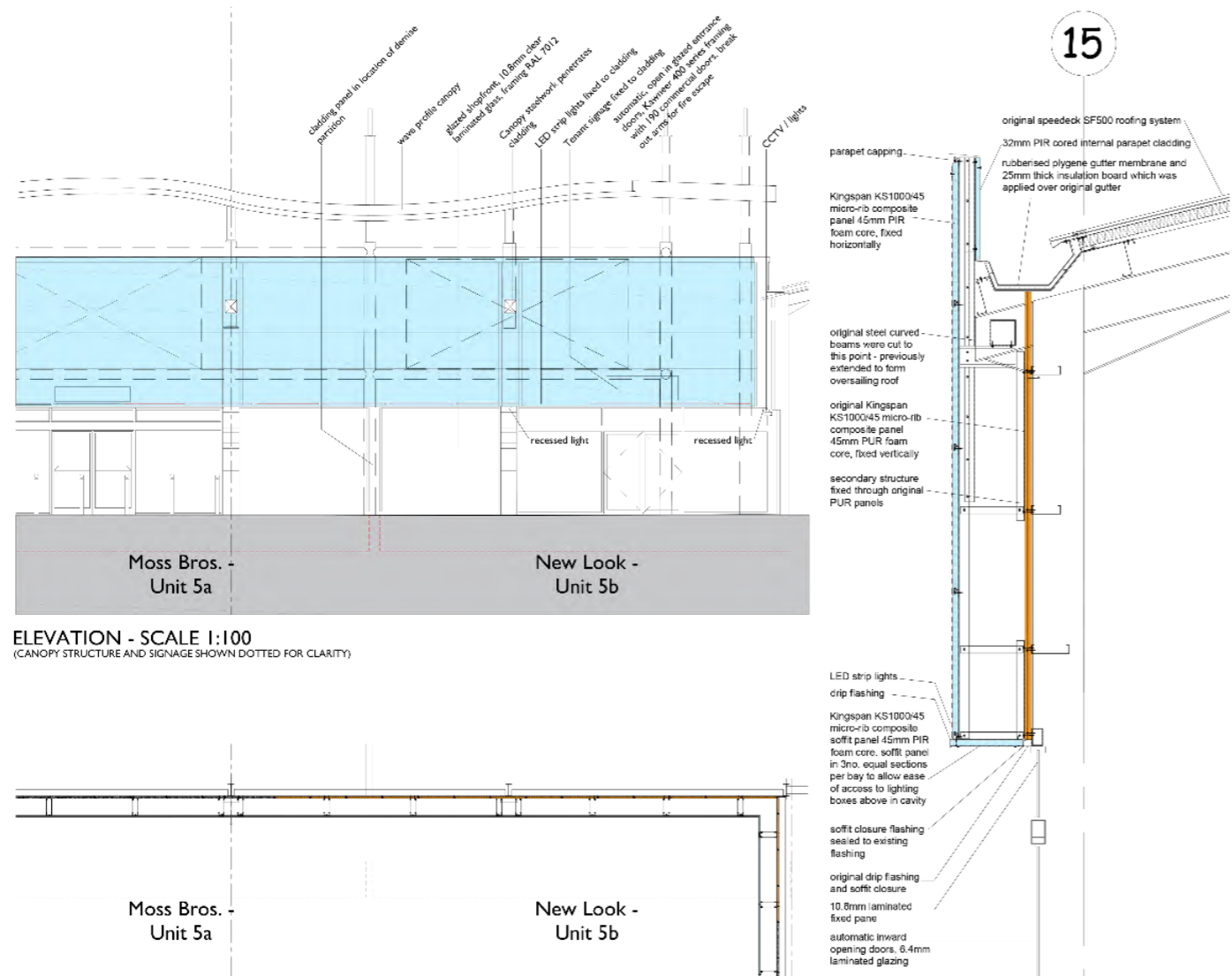
Plan through cladding
